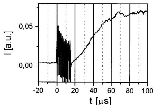
FIG. 4. The switching rate of the FLC shutter is monitored by opening the shutter using a constant probe intensity. The fluorescence intensity I(t) reveals a delay time of \sim 15\ \mu\text{s} and a rise time (for a change from 10% to 90% of the final value) of 55\ \mu\text{s} .
