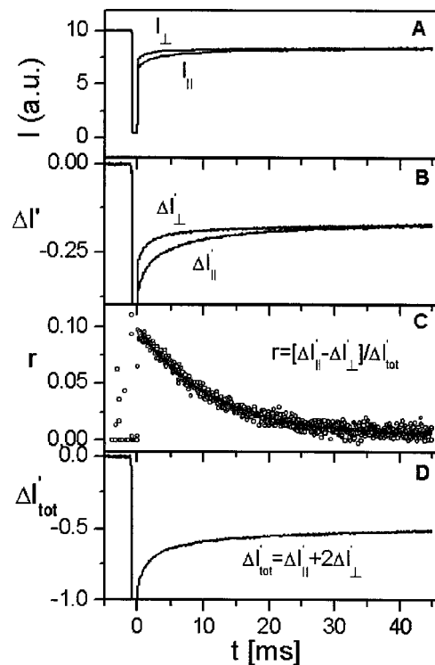
FIG. 5. Photobleaching measurement of the rotational diffusion of rhodamine-labeled SiSol particles ( a_T=230 nm, volume fraction of 0.1%) in DMF. Curves are averages over 128 runs measured at different places in the sample. (A) The fluorescence intensity induced by the probe beam as a function of time. (B) The normalized bleach contrast according to Eq. (38). (C) The anisotropy, with the solid line denoting a best exponential fit. (D) The total normalized bleach contrast.
