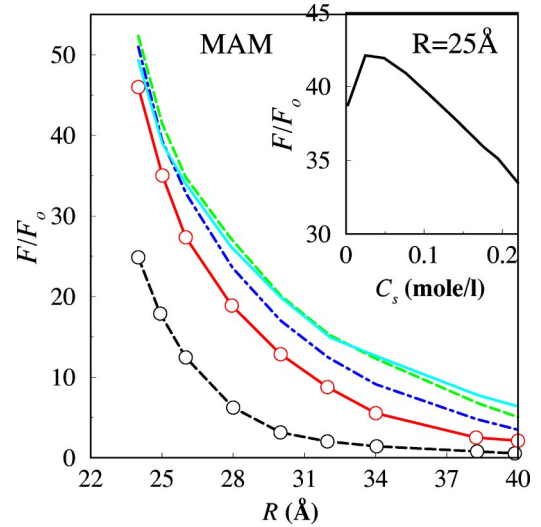
FIG. 4. (Color online) Reduced DNA-DNA interaction force F/F_0 vs separation distance R for the monovalent counterions and monovalent salt ions (parameter set 1 of Table I) for the MAM. The CM and ECM exhibit similar trends. The unit of the force is F_0 = k_B T/P , where P is the DNA pitch length. Different salt densities are shown: C_s = 0 mole/l (solid line), 0.024 mole/l (dashed line), 0.097 mole/l (dot-dashed line), 0.194 mole/l (solid line with symbols), 0.71 mole/l (dashed line with symbols). The corresponding screening lengths are \lambda_D = 9.6 \text{ \AA} , 9 \text{ \AA} , 8 \text{ \AA} , 5.6 \text{ \AA} , 3.3 \text{ \AA} . The inset shows the force-salt nonmonotonicity at the separation distance R = 25 \text{ \AA} .
