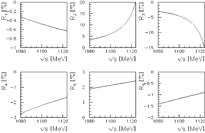
FIG. 4. Isospin violation in the P_1 -wave projection of the ratios R_1 – R_6 .
