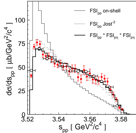
Fig. 3. Experimental distribution of the square of the proton-proton invariant mass ( s_{pp} ) determined experimentally for the pp \rightarrow pp\eta reaction at the excess energy of Q = 15.5 \text{ MeV} by the collaborations COSY-11 [14] (closed circles) and TOF [15] (open circles). The TOF data have been normalized to give the same total cross section as those of the COSY-11. The integral of the phase space weighted by the proton-proton on-shell scattering amplitude and by the inverse of the proton-proton squared Jost function [16] is represented by the thin solid and dashed line, respectively. The thick solid line shows the result of the calculations where the occupation density of the phase space was weighted by the inverse of the Jost function multiplied by the square of the proton- \eta scattering amplitude. The latter was calculated taking arbitrarily the scattering length a_{p\eta} = 0.7 \text{ fm} + i0.4 \text{ fm} . The lines have been normalized in amplitude to the data.
