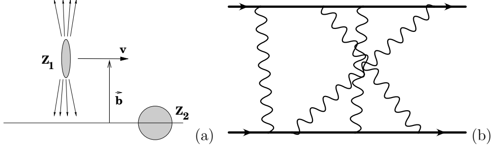
Fig. 1. a) Classical picture of heavy ion scattering. This picture was also used by Fermi in his celebrated paper on the equivalent photon approximation [18]. He considered the nonrelativistic case v \ll c . The relativistic case is discussed in a very pedagogical manner in [14]. (b) For \eta \gg 1 many photons are exchanged in elastic heavy ion scattering. A typical graph is shown.
