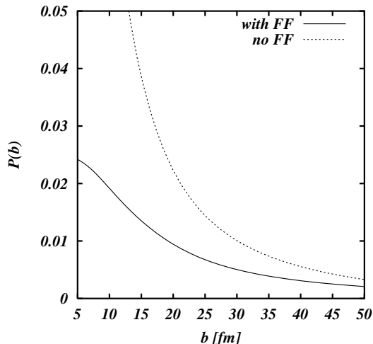
Fig. 4. The probability of muon pair production is shown as a function of impact parameter for Pb-Pb collisions at the LHC ( \gamma = 3400 ). Results for a monopole form factor F(Q) = 1/(1 + Q^2/\Lambda^2) with \Lambda = 83 MeV and without a form factor ( F(Q) = 1 ) are given.
