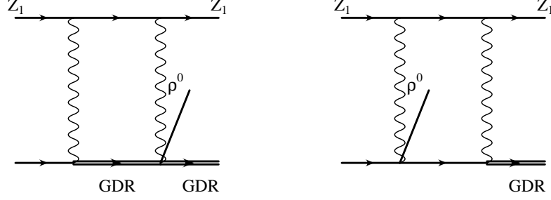
Fig. 2. Graphs contributing to the simultaneous excitation of states \alpha and \beta . In this figure we take \alpha = GDR and \beta = \rho^0 as a typical example.
