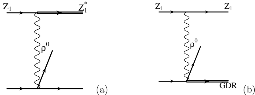
Fig. 3. Examples of graphs which spoil the factorization of the different processes, compare also with the figure above. As discussed in the text their contribution are expected to be small.
