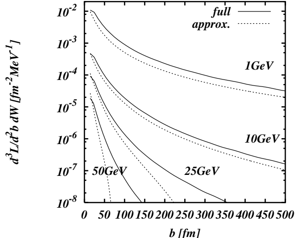
Fig. 6. The photon-photon luminosity d^3L/d^2bdW is shown for different values of W as a function of the impact parameter b . The results of a full calculation for lead beams at the LHC are compared with the approximate result of Eq. (54).
