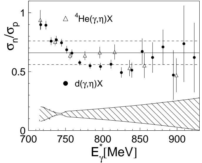
Fig. 8. Ratio of neutron and proton cross section as function of the equivalent photon energy for the deuteron and for {}^4\text{He} [17]. The lines indicate the average extracted from the exclusive cross sections as function of the incident photon energy. The shaded band represents the systematic uncertainty of the ratio due to the relative calibration of the proton and neutron recoil energies.
