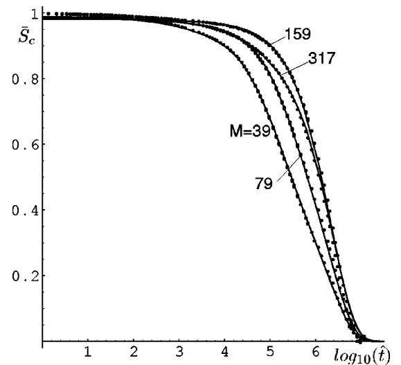
FIG. 9. Results for \bar{S}_c, q=0.5, N=317 . Theoretical results (solid lines) for central subchains of lengths M=39, 79, \text{ and } 159 are compared to simulations (dots). Results for the total chain ( M=317 ) are also shown.
