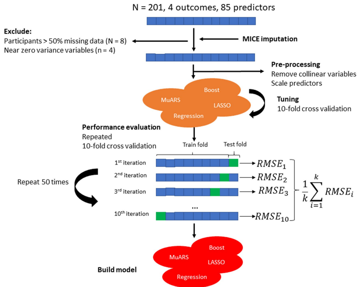
Figure 2. Predictive modelling workflow. RMSE root mean squared error, MuARS multivariate adaptive regression spline, lm linear regression, LASSO least absolute shrinkage and selection operator, MICE multivariate imputation by chained equations.
