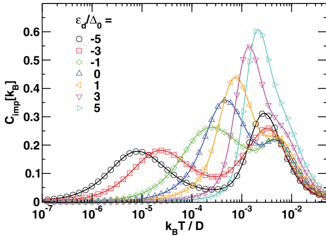
FIG. 10. (Color online) Temperature dependence of C_{\text{imp}}(T) for U/\Delta_0 = 12 , \Delta_0 = 0.001D , and local level positions \varepsilon_d/\Delta_0 ranging from Kondo ( \varepsilon_d/\Delta_0 \leq -1 ), mixed valence ( |\varepsilon_d/\Delta_0| \leq 1 ), and empty orbital ( \varepsilon_d/\Delta_0 > 1 ) regimes. Symbols: NRG calculations (new approach, z averaging, and NRG parameters as in Fig. 1). Lines: Bethe ansatz calculations.
