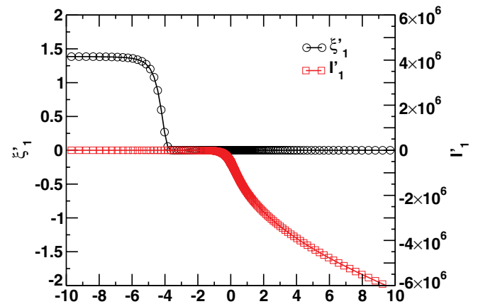
FIG. 15. (Color online) Comparison between I'_1 and \xi'_1 for 500 iterations and T = 10^{-4} T_K . Parameters were chosen to be the same as in Fig. 1. For very low temperatures \xi'_1 (circles, left y axis) exhibits an exponential drop beyond a certain rapidity \Lambda_0 ( \approx -4 for the case shown), which is difficult to capture with a fixed grid. This problem can be overcome by using the smooth function I'_1 (squares, right y axis) to calculate \xi'_1 via Eq. (B4c).
