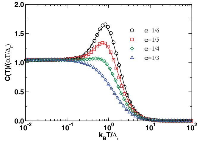
FIG. 13. (Color online) Specific heat C_{\text{imp}}(T)/(\alpha k_B T/\Delta_r) of the Ohmic two-state system as a function of reduced temperature k_B T/\Delta_r for a range of dissipation strengths \alpha < 1/2 . Symbols: NRG results in new approach. Lines: Bethe ansatz results. In the low-temperature Fermi liquid regime T \ll \Delta_r we have C_{\text{imp}}(T)/(\alpha k_B T/\Delta_r) = \tilde{\gamma} + \tilde{\beta}(T/\Delta_r)^2 , with \tilde{\gamma} = \pi/3 and the T^3 coefficient in C(T) changes sign for \alpha < 1/3 (see Ref. 62). Model parameters: \Delta_0/\omega_c = 0.005 . NRG parameters: \Lambda = 10, n_z = 4 retaining 860 states per NRG iteration.
