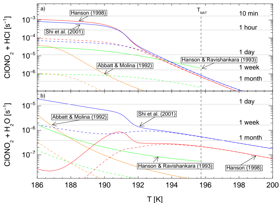
Fig. 1. First order loss rates for \text{ClONO}_2 + \text{HCl} (a) and \text{ClONO}_2 + \text{H}_2\text{O} (b) for different parameterizations and aerosol types for typical stratospheric conditions (50 hPa, 5 ppmv \text{H}_2\text{O} , 1 ppbv HCl, 0.5 ppbv \text{ClONO}_2 , 10 ppbv \text{HNO}_3 , 0.15 ppbv \text{H}_2\text{SO}_4 and 10 background aerosol particles \text{cm}^{-3} ). Solid red and blue lines depict ternary aerosol, dashed lines binary aerosol. Solid green and orange lines represent NAT particles with density 10^{-1} \text{ cm}^{-3} , dashed lines 10^{-4} \text{ cm}^{-3} . Adapted from Dameris et al. (2007).
