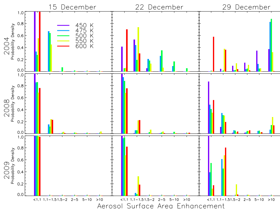
Fig. 7. Probability density distribution of maximum surface area density enhancement by STS along 7 day back-trajectories starting on MLS observations poleward of 75^{\circ} N equivalent latitude.
