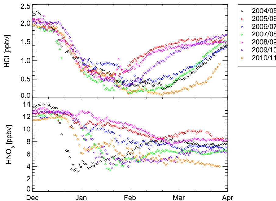
Fig. 6. HCl and HNO 3 observations by MLS for the Arctic winters 2004/2005 to 2010/2011 on 500 K potential temperature in the vortex core (equivalent latitude > 75° N).
