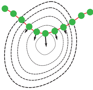
FIG. 3. (Color online) If S \rightarrow 0 , \mathbf{F}_{13} can only move the images along the band but cannot change its shape, and the band cannot escape from the minimum.
