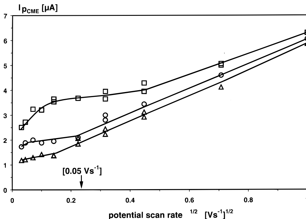
Figure 2. Effect of the potential scan rate on the reduction current intensity of \text{Fe}(\text{CN})_6^{3-} for various CME coatings in 4 M NaCl solution. □, CME coating 0.28 mg/cm 2 ; ○, CME coating 0.56 mg/cm 2 ; △, CME coating 1.13 mg/cm 2 ; \text{K}_3\text{Fe}(\text{CN})_6 , 4 mM; Na-montmorillonite I.
