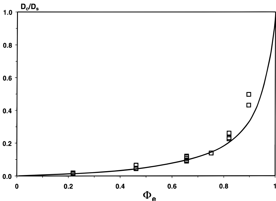
Figure 5. Dependence of the relative variation of Fe(CN)_6^{3-} diffusion coefficient at CME, R^2 = D_c/D_s on the effective porosity \Phi_e (calculated with eq 6). The curve is calculated with eq 7 where the shape factor \alpha = 17.8 (see also text).
