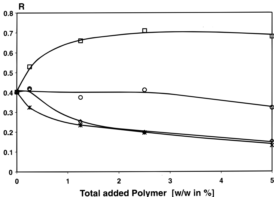
Figure 9. Effects of the water-soluble polymer content (w/w) of CME on the cyclic voltammogram intensity current ratios R = I_{\text{PCME}}/I_{\text{Psol}} of \text{Fe}(\text{CN})_6^{3-} in 0.2 M NaCl solution. \circ , PVP (MW 5000 g/mol); * , PVP (MW 44 000 g/mol); \diamond , PVP (MW 400 000 g/mol); \square , PAA (MW 2000 g/mol); Na-montmorillonite II.
