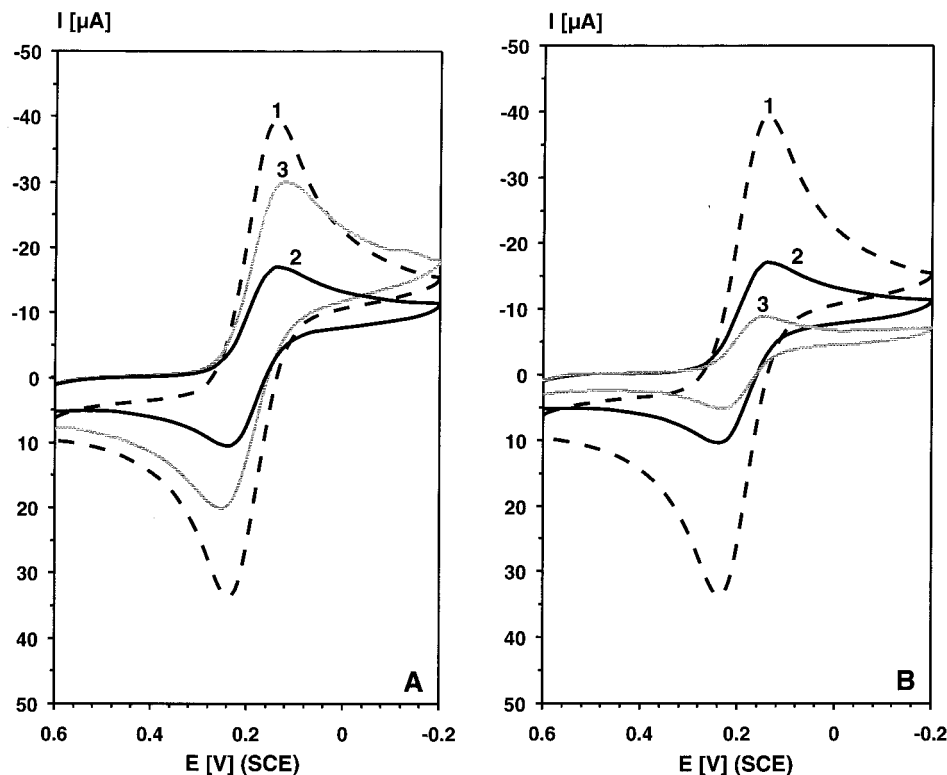
Figure 8. Cyclic voltammograms of \text{Fe}(\text{CN})_6^{3-} at polymer-modified CME (w/w: 5%) in 0.2 M NaCl solution. A: 1, bare-Pt electrode; 2, unmodified CME; 3, PAA (MW 2000 g/mol)-modified CME. B: 1, bare Pt electrode; 2, unmodified CME; 3, PVP (MW 44 000 g/mol)-modified CME. Potential scan rate 0.05 V/s; CME coating 1.13 \text{ mg/cm}^2 ; \text{K}_3\text{Fe}(\text{CN})_6 , 4 mM; Na-montmorillonite II.
