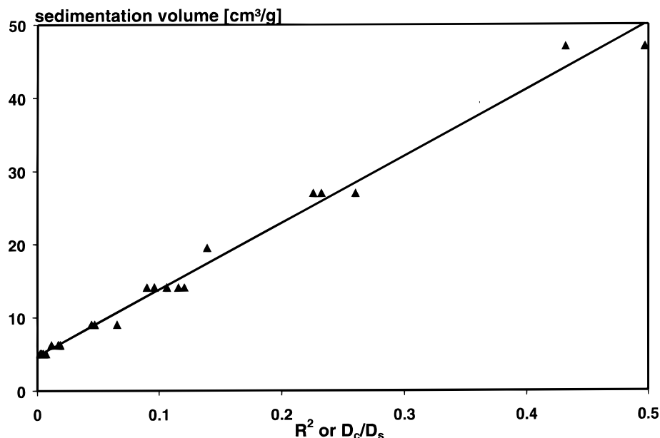
Figure 4. Relationship between the sedimentation volumes and the relative variation of the Fe(CN)_6^{3-} diffusion coefficient at CME expressed in R^2 = D_c/D_s , (see also Figure 3).
