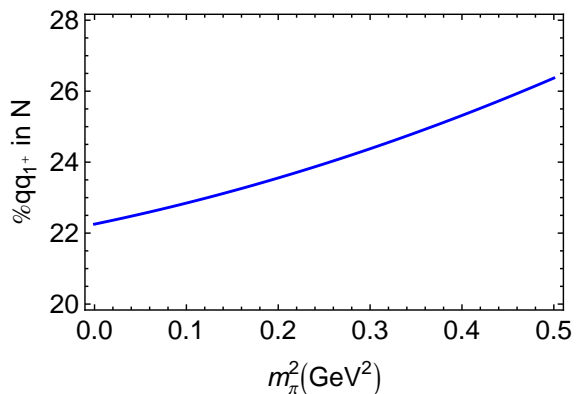
Fig. 6 Evolution with current-quark mass of the contribution made by axial-vector-diquark correlations to the unit-normalisation of the nucleon’s Faddeev amplitude. At the model-preferred current-quark mass, the probability is 22%. This rises to 26% at m = m_s .
