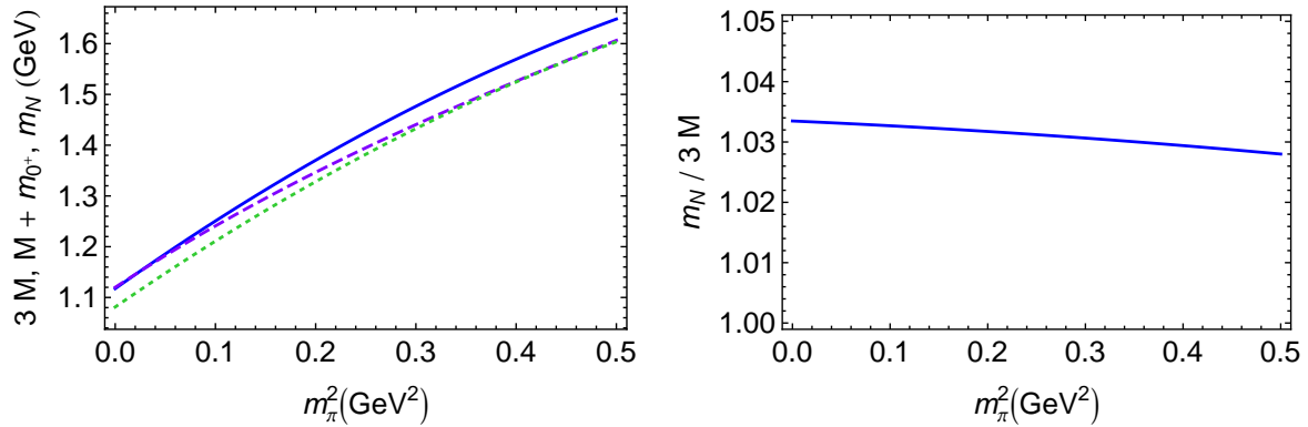
Fig. 3 Left panel – Evolution with current-quark mass of the: nucleon mass, m_N (solid curve); the sum [M + m_{q_{0+}}] (dashed curve); and 3M (dotted curve). Right panel – Evolution with current-quark mass of the ratio m_N/[3M] , which varies by less-than 1% on the domain depicted.
