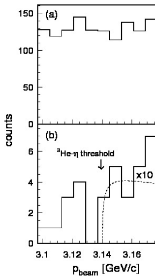
Fig.2. Number of dp \rightarrow ppp\pi^- events as a function of the beam momentum without any cuts (a) and after rejection of events corresponding to the quasi-free \pi^- production (b). The dashed line represents calculations of the \eta absorption described in the text.
