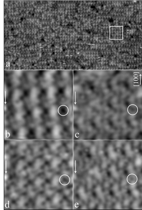
FIG. 4. (a) 70 \times 35 \text{ nm}^2 STM image recorded on a terrace for V_b=2 \text{ V} and I_t=0.06 \text{ nA} . The white frame outlines a patch of homogeneous contrast. [(b)–(e)] STM images ( 5.1 \times 5.1 \text{ nm}^2 ) acquired on the same region using a constant current of 40 pA and a bias of (b) 0.8 V, (c) -0.8 V, (d) 0.4 V, and (e) -0.4 V. The arrows point to a common defect visible on all images. As shown by the circles located at the same position on all images, the contrast varies drastically with the applied bias.
