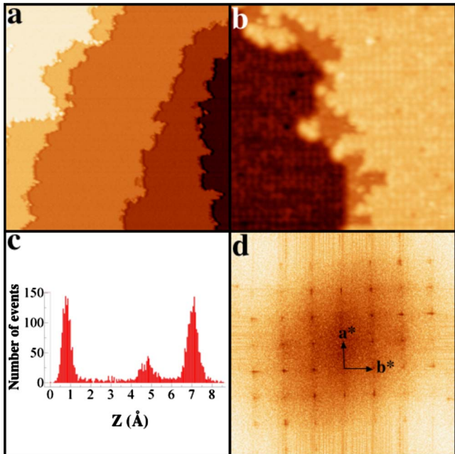
FIG. 3. (Color online) (a) STM image ( 250 \times 250 \text{ nm}^2 ) showing the step and terrace morphology. (b) STM image ( 40 \times 40 \text{ nm}^2 ) showing a narrow terrace on the step edge. (c) The height histogram calculated from a 20 \times 20 \text{ nm}^2 STM image exhibits the three possible step heights observed across terraces. (d) Fast Fourier transform calculated from a 50 \times 50 \text{ nm}^2 high-resolution STM image.
