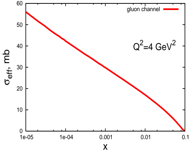
Figure 10. The effective gluon shadowing cross section, \sigma_{\text{eff}}^g(x) , at Q^2 = 4 \text{ GeV}^2 as a function of x for the H1 parameterizations of the diffractive gluon density.
