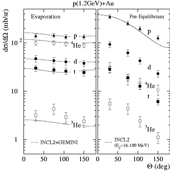
Fig. 4. Angular distributions of ^{1,2,3}\text{H} and ^{3,4}\text{He} for 1.2 GeV p+Au. symbols: exp. data, lines calculation by INCL2.0+GEMINI; [9]
