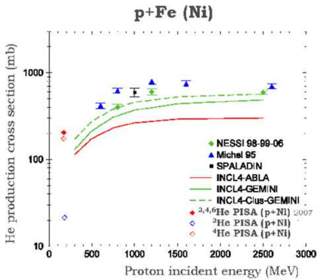
Fig. 6. Production cross section of {}^{3,4,6}\text{He} isotopes as a function of incident proton beam energy. symbols: NESSI,Hannover,SPALADIN,PISA data, curves: calculation by INCL4.3+GEMINI/ABLA
