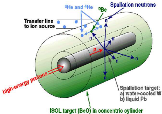
Fig. 1. {}^6\text{He} -production by converter technology using spallation neutrons.
