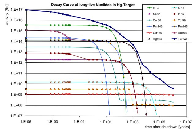
Fig. 2. Decay curves of long lived nuclides in Hg-target which determine the activity during operation and after 30years of 5 MW operation.
