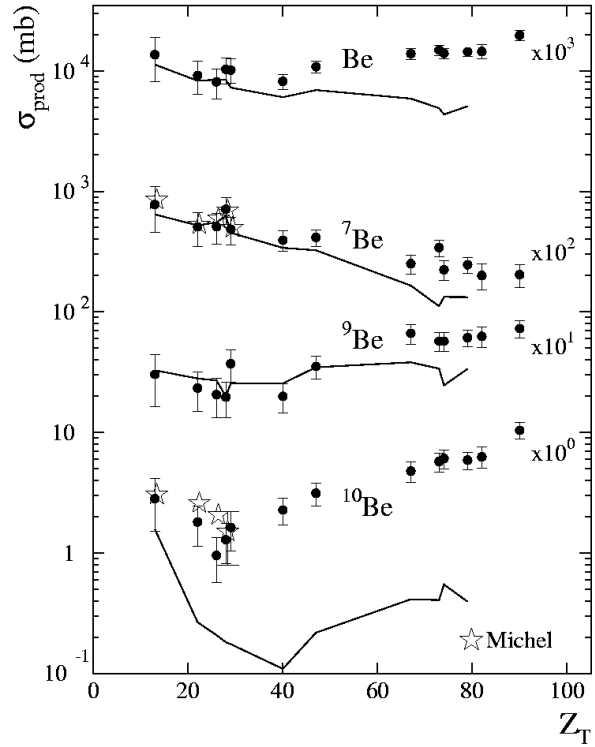
Fig. 5. Production cross section of ^{7,9,10}\text{Be} isotopes for 1.2 GeV p+X. •: NESSI [9], ★: R. Michel [13] data, lines: calculation by INCL2.0+GEMINI
