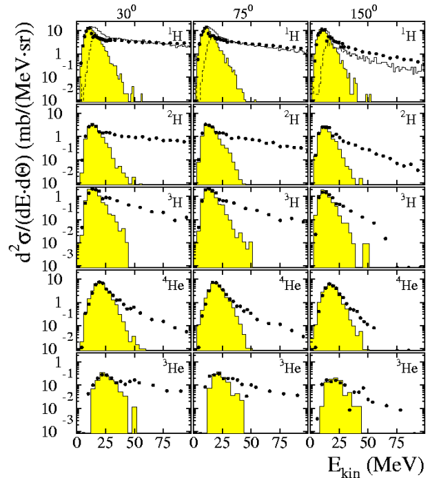
Fig. 3. Energy spectra of ^1,2,3\text{H} and ^3,4\text{He} for 1.2 GeV p+Ta. dots: exp. data, shaded hist.: calculated evap. spectra, dashed hist.: pre-equilibrium protons as calculated by INCL2.0; [9]
