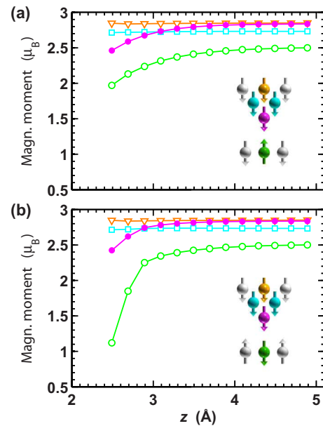
FIG. 11. (Color online) Distance dependence of the magnetic moments of different Fe atoms of the fourteen-atom tip—apex (closed circles), base second layer (open squares), and center atom of third layer (open triangles)—and the surface Fe atom (open circles) of the Fe ML on W(001) for (a) ap and (b) p alignments between the magnetization of tip and surface atom as shown in the insets without structural relaxations of tip and sample.
