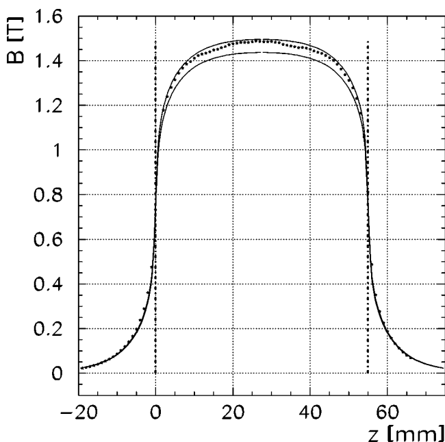
FIG. 11. Magnetic flux density B_{\text{rad}} ( \star ) along the axis of magnet 6 at a radius of 14.5 mm at \phi=0 . The upper solid line indicates the result of a MAFIA calculation using typical values for the remanence J^{\text{yp}} of the individual segments (Table I). The lower solid line for the configuration with minimal values of the magnetization is obtained by scaling the results obtained with J^{\text{yp}} by a factor J^{\text{min}}/J^{\text{yp}} . The dashed lines correspond to the physical boundaries of the magnet.
