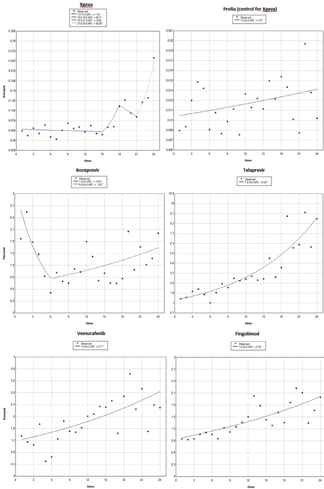
FIGURE 3 Jointpoint regression analysis—new products included in the study. Reporting of post-marketing ADRs from the EEA, addition to AM list is at time point 12 (time in months)
