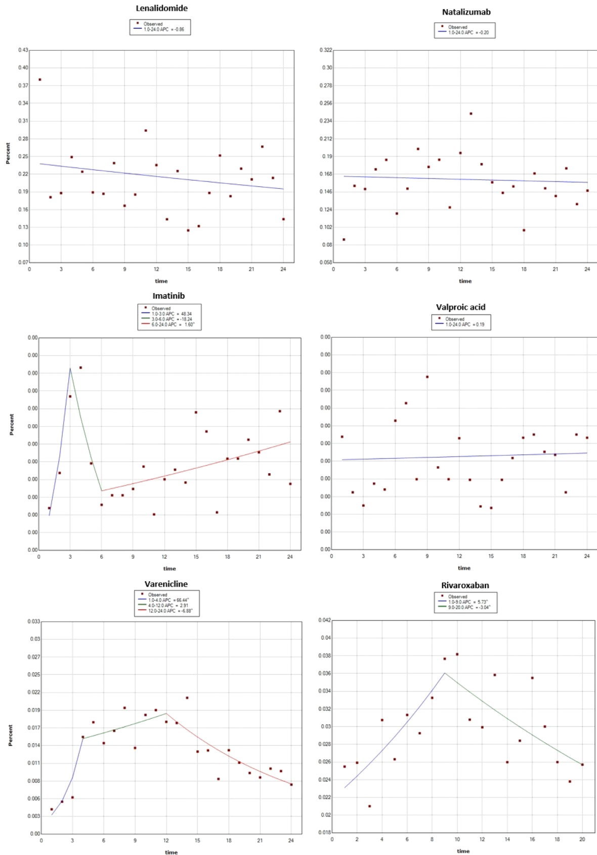
FIGURE 4 Joinpoint regression analysis—products included in the study due to PASS requirement. Reporting of post-marketing ADRs from the EEA, addition to AM list is at time point 12 (time in months)
