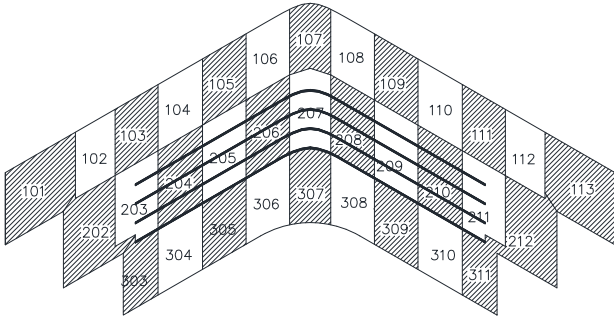
Figure 2: Partitioning scheme for steel truss roof.
