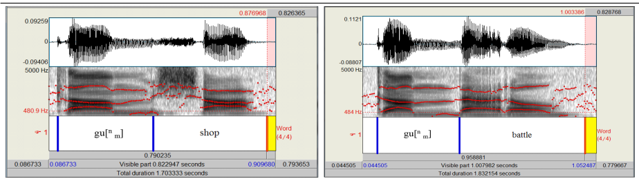
Figure 1. The waveforms and spectrograms of ‘gu [n m] shop’ in the unviable change context and ‘gu [n m] battle’ in the viable change context
