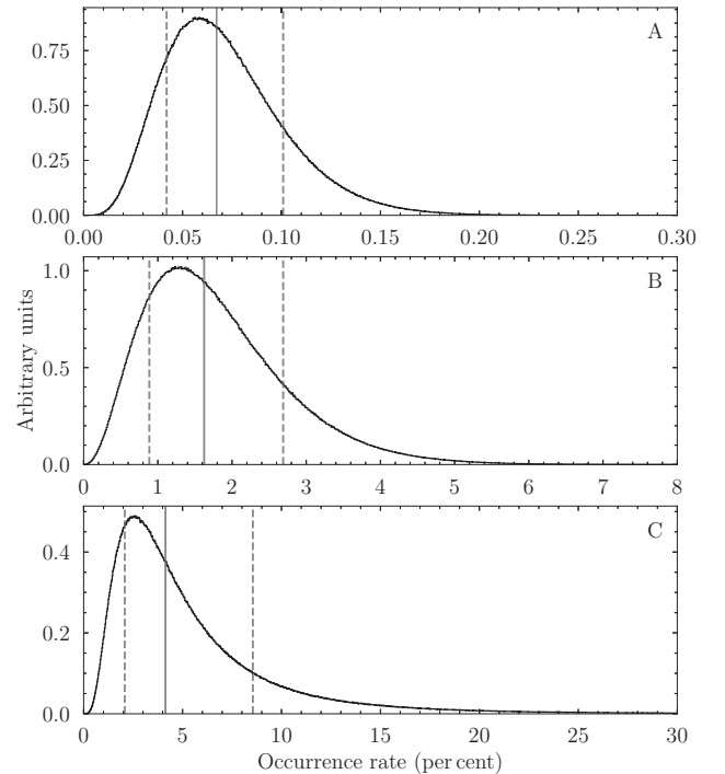
Figure 4. Histograms evaluated from the probability distributions of the occurrence rates of (A) debris discs with a gaseous component in emission around white dwarfs, (B) dusty debris discs around white dwarfs, and (C) a gaseous component to a debris disc in emission. The solid grey lines represent the median value of the distributions, and the dashed lines mark the 15.9 and 84.1 percentiles corresponding to \pm 1\sigma . (A) [(B)] is constructed from 10 million evaluations of equation (3) using n = 5 [3], and t = 7705 [195]. (C) is produced by dividing each evaluation of (A) by a corresponding evaluation of (B).
