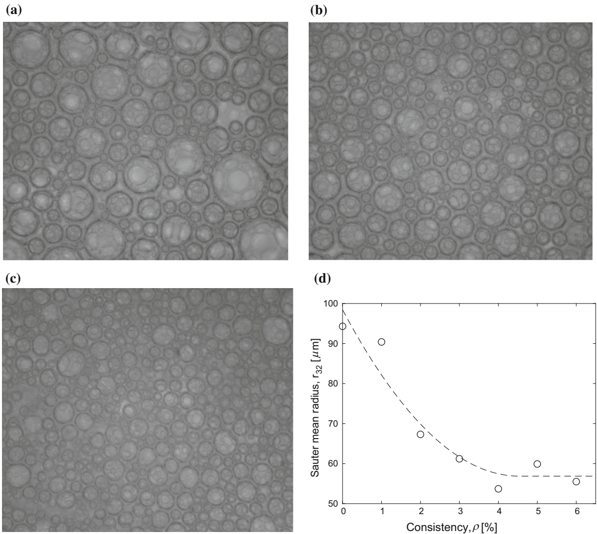
Fig. 1 Microscopic images (1.7 mm \times 2.0 mm) of aqueous foam samples taken from the mixing tank: a Pure foam. b Fiber consistency 2.0%. c Fiber consistency 6.0%. d Sauter mean
