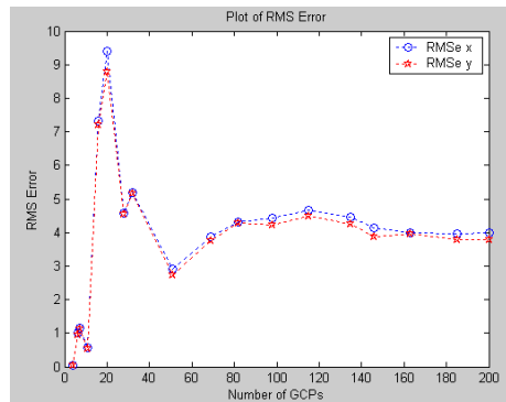
Figure 5. RMSe (m) of random error data on flat terrain
