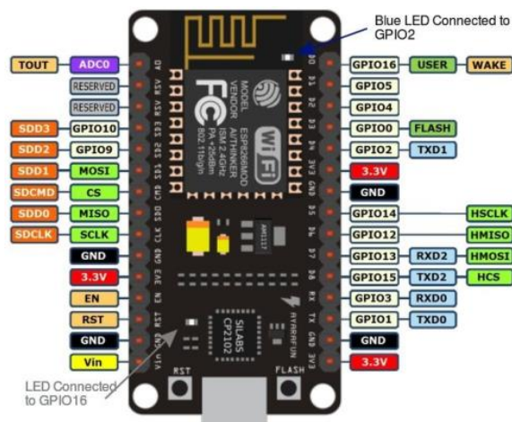
Gambar 3. Diagram pin NodeMCU [10]
