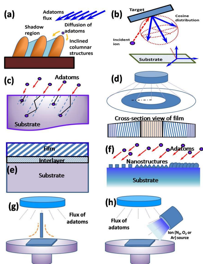
Figure 6. (a) Illustration of the shadowing effect during film deposition; (b) Cosine law distribution of the sputtered adatoms on the substrate surface; (c) channelling effects during sputtering process; (d) A circular-shaped target produces a ring distribution of inclined columnar angles (dark area) in the films, which can be revealed clearly from the illustration of cross-section morphology; (e) An interlayer can promote the growth of inclined angled films; (f) Pre-treatment of surface to generate the desired surface roughness or surface topography and enhance shadowing effect for growth of inclined angled films; (g) An additional blind/shutter positioned between the target and the substrates can change the plasma distribution onto the deposited films, thus promoting the inclined film growth; (h) An external oxygen or nitrogen ion or plasma source can control the oxygen/nitrogen ion bombardment to the deposited film during its inclined angled film growth.
