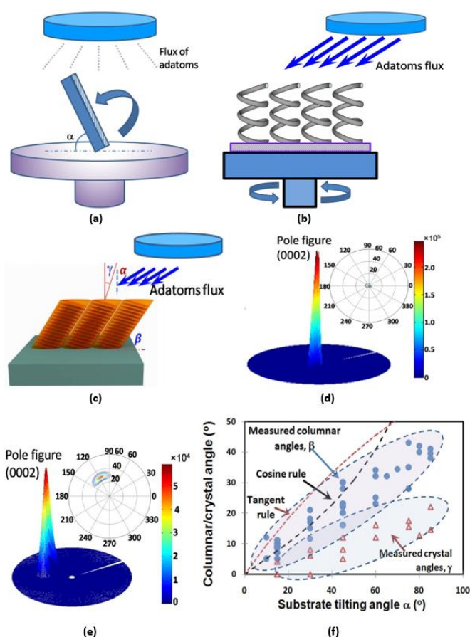
Figure 5. (a) Tilting angle deposition or oblique angle deposition (OAD); (b) Glancing angle deposition (GLAD) with tilting/rotating in a 3D scheme at very large tilting angles; (c) Illustration of the relationship between columnar tilting angle, substrate tilted angle and crystal tilting angles; (d) X-ray diffraction (XRD) pole figures of a c-axis orientated AlN films; (e) XRD pole figures of a 30° crystal inclined AlN films; both figures (d) and (e) are provided by Prof. Enrique Iborra from University of Polytechnic Madrid, Spain; (f) Different angles readings along with the data produced from the tangential and cosine rules 5 . Here, the adatoms refer to the arriving and deposited atoms/ions onto the substrate surface, and they are originated from the sputtering targets through diffusion, migration and bombardment.
