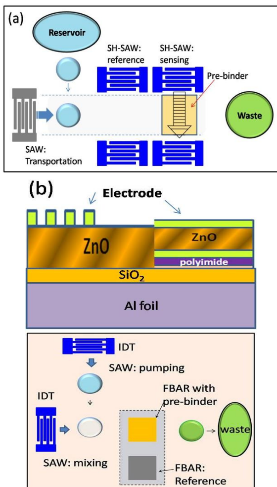
Figure 9. (a) Integrated liquid sensor using both Rayleigh mode SAW and SH-SAW on substrate; (b) demonstration of a smart and integrated system based on SAW biosampling and liquid transportation functions and FBAR liquid sensing functions.
