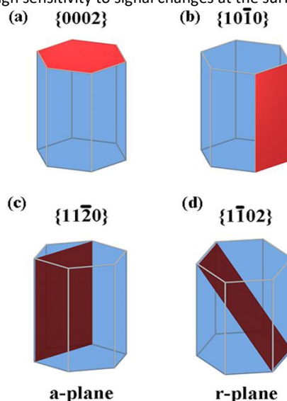
Figure 2. Illustrations of four commonly observed orientations for wurtzite piezoelectric crystal structures. (a) {0002}c-plane; (b) \{10\bar{1}0\} m-plane; (c) \{11\bar{2}0\} a-plane; and (d) \{1\bar{1}02\} r-plane.
