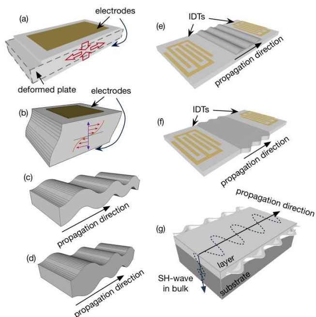
Figure 1. Illustrations of different types of commonly observed acoustic waves: including (a) longitudinal bulk acoustic waves (BAWs) generated between a top electrode and bottom electrode; (b) thickness-shear mode (TSM) waves generated between two electrodes; (c) Lamb waves, antisymmetric mode (A mode, or flexural plate waves-FPWs); (d) Lamb waves, symmetrical mode or extensional mode (S mode); (e) Rayleigh surface acoustic wave (SAW) generated on a piezoelectric materials using interdigital transducer (IDTs); (f) shear horizontal SAWs (SH-SAWs) generated on piezoelectric materials using IDTs; (g) Love-mode wave modes generated on the surface of an SH-SAW device coated with a thin wave-guide layer.
