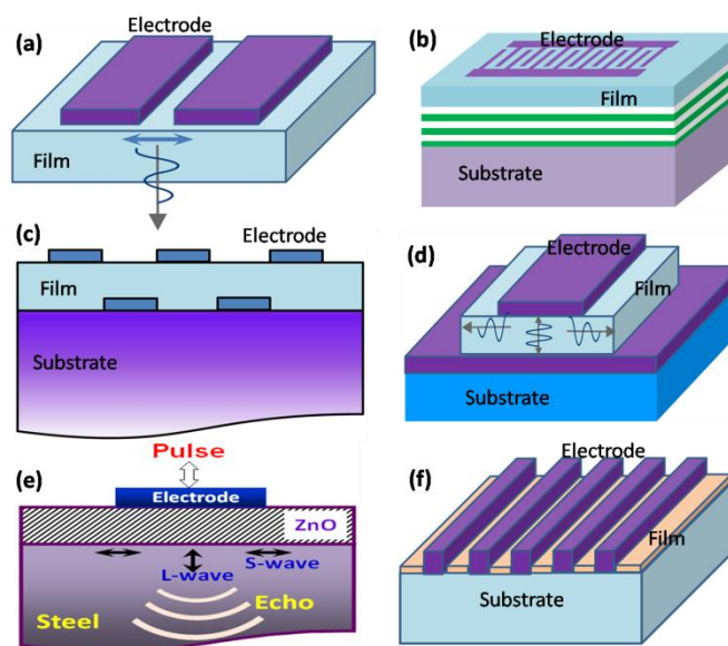
Figure 4. The acoustic waves are excited in different structures: (a) lateral field electrode to form laterally excited ZnO or AlN thin film resonators to generate shear waves to be operated in a liquid solution; (b) tilt electric fields generated from standard IDTs on a c-axis vertically aligned piezoelectric film deposited on dielectric reflector stacks of AlN/SiO 2 , thus resulting in the electric fields mainly aligned along the x-axis of the film plane; (c) the top and bottom electrodes are not perfectly aligned in z-direction, thus the asymmetrical fields will generate both vertical and shear waves; (d) off-axis excitation, where the top electrode is relatively smaller than the bottom electrode thus both pseudo-shear and pseudo-longitudinal waves can be generated; (e) both longitudinal wave (L-wave) and shear bulk wave (S-wave) generated in a standard pulse-echo ultrasonic test; (f) a periodically patterned ZnO film was deposited between fingers of IDTs to fill the gaps of the IDTs and implement SAW resonators.
