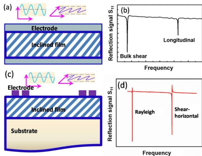
Figure 3. The configurations of thin films and acoustic waves that can be generated: (a) Thin film FBARs with inclined angled piezoelectric thin films can generate both longitudinal (for microfluidics) and bulk shear waves (for liquid sensing); (b) A schematic illustration to indicate the differences in the frequencies of longitudinal and bulk shear waves; (c) Rayleigh SAW and SH-SAW generated with IDTs deposited on top of inclined angled piezoelectric films; (d) A schematic illustration to indicate the differences in the frequencies of Rayleigh SAW and SH-SAWs.
