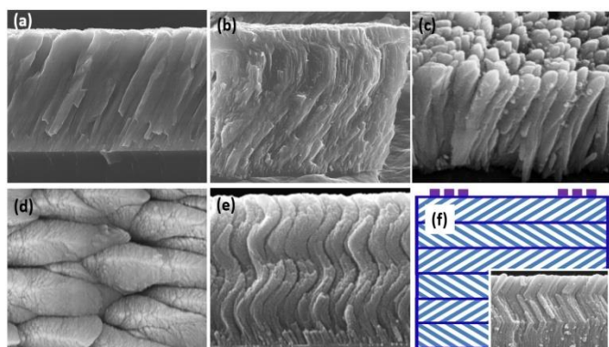
Fig. 7. (a) An inclined angled ZnO films with a thickness of 3.5 microns on silicon; (b) columnar inclination angles of films with columnar inclined angle has gradually changed during deposition; (c) porous and loose columnar inclined microstructures; (d) rough and significantly elongated surface grainy structures for columnar inclined angled ZnO films; (e) Example of 3D spiral and porous nanorods structures fabricated from GLAD methods; (f) Illustration and example of multi-layered zig-zag ZnO structures.
