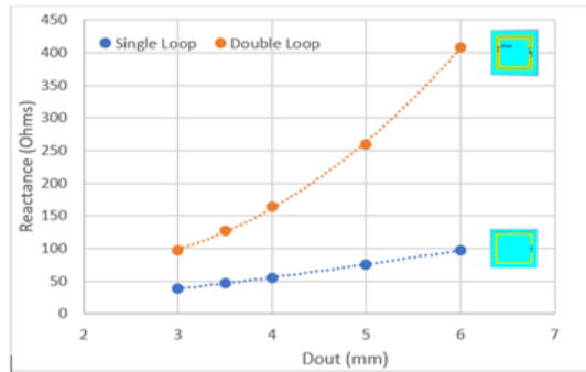
Figure 3 Single and double loop reactance.
