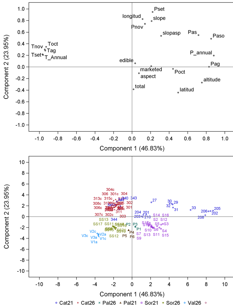
Fig. 1 Scatterplots of the loadings (above) and the scores (below) obtained by PCA applied on plots. In parentheses are shown the percentage of variability accounted by the two first components. “total” denotes all ectomycorrhizal mushrooms yield, “edible” denotes edible mushrooms yield, “marketed” denotes marketed mushrooms yield, “altitude” denotes the plot altitude, “latitud” denotes the plot latitude, “longitud” is denotes the plot longitude, “slope” denotes the main slope of the plot, “aspect” denotes the plot aspect, “slopeasp” is a synthetic variable created by multiplying slope by aspect, “P_annual” is the annual accumulated precipitation, “P_ag” is the accumulated precipitation of August, “P_set” is the accumulated precipitation of September, “P_oct” is the accumulated precipitation of October, “P_nov” is the accumulated precipitation of November, “P_as” is the accumulated precipitation of August and September, “P_aso” is the accumulated precipitation of August, September and October, “T_annual” is the annual mean temperature, “T_ag” is the mean temperature of August, “Tm_set” is the mean temperature of September, “T_oct” is the mean temperature of October, “T_nov” is the mean temperature of November, 21 is Pinus sylvestris and 26 is Pinus pinaster , Cat is Catalonia region, Pal is Palencia province, Sor is Soria province and Val is Valladolid province
