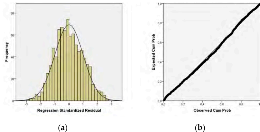
Figure 1. Multiple linear regression (MLR) assumptions. (a) Regression Standardized Residual; (b) Observed Cum Prob.
