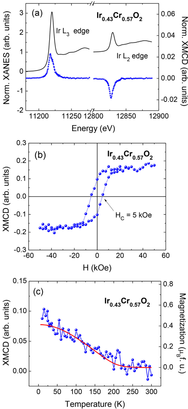
Fig. 8. (a) Normalized XANES and XMCD spectra recorded at the Ir L 2,3 edges at T = 10 K and H = 50 kOe on polycrystalline Ir 0.43 Cr 0.57 O 2 sample. (b) Ir L 3 -edge field-dependent XMCD curve at T = 10 K and E = 11,218 eV. (c) Ir L 3 -edge temperature-dependent XMCD curve with H = 1 kOe. The FC-M(T) is also included for comparison.
