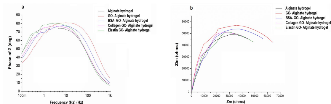
Figure 7. Electrochemical study from protein coated-GO alginate hydrogels compared to alginate hydrogels. (a) Bode plots, (phase angle Z vs. frequency from 10^{-1} to 10^3 Hz). (b) Nyquist diagram, Zim vs. Zre (ohm).
