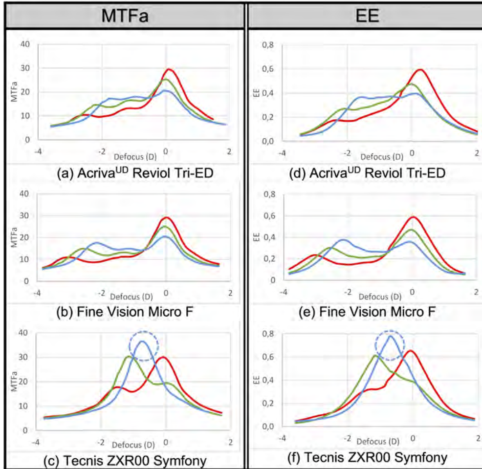
Fig. 1. R, G and B through-focus MTFa (left column) and EE (right column) curves obtained with a 3.0 mm pupil for three IOLs: trifocal Acryva Reviol Tri-ED (a, d), trifocal FineVision Micro F (b, e), and ERV Tecnis ZXR00 Symphony (c, f). Blue, green and red solid lines correspond to blue (455 nm), green (530 nm) and red (625 nm) illumination, respectively. Dashed circles in (c, f) indicate the peak values of blue MTFa and EE of the Symphony IOL (see text for details).
