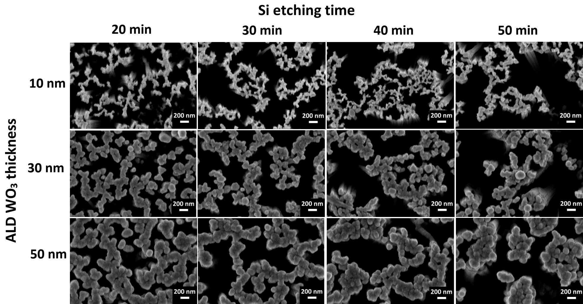
Figure S2: SEM images of \text{WO}_3/\text{Si} nanowires fabricated with different Si etching time: 20 min, 30 min, 40 min and 50 min, and coated \text{WO}_3 films with different thickness: 10 nm, 30 nm, 50 nm.
