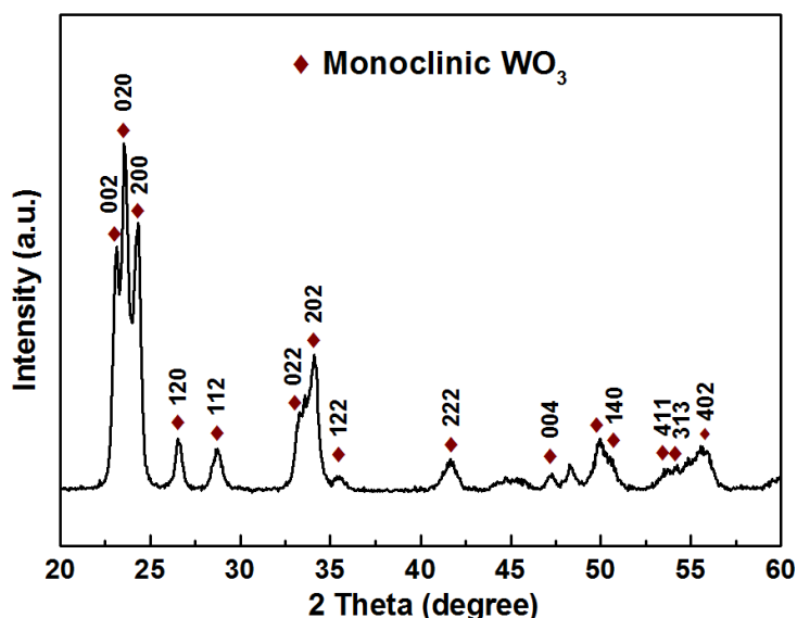
Figure S3: GIXRD spectra of Si nanowires (50 min etching) coated WO 3 (50 nm) after annealing in Ar. (monoclinic WO 3 corresponding to JCPDS No. 83-0950)
