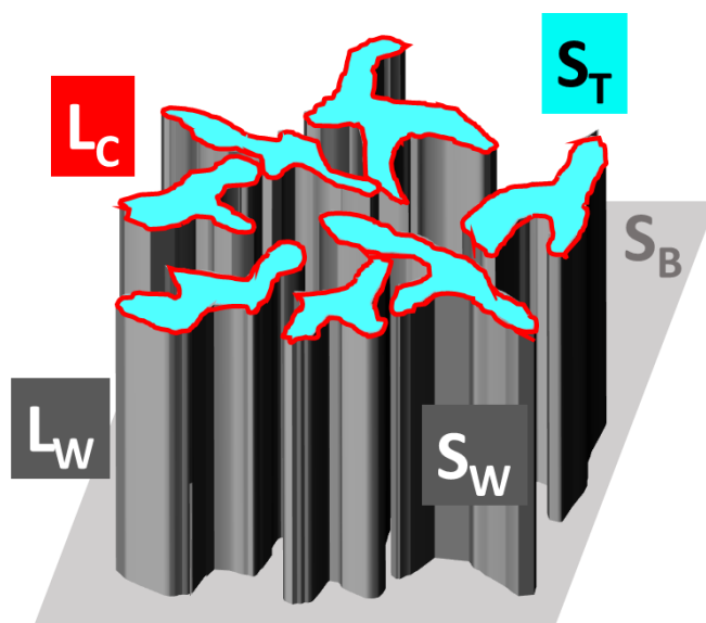
Figure 3. Sketch of the geometry of the \text{WO}_3/\text{Si} nanowires ( S_T : top surface area; L_C : length of the contour of the top surface; L_W : length of the nanowires; S_W : wall surface area; S_B : bottom surface area.)
