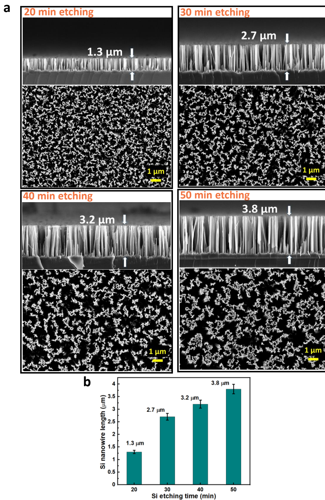
Figure S1: (a) Scanning electron microscope (SEM) images of Si nanowires fabricated with different etching time: 20 min, 30 min, 40 min and 50 min. (b) Si nanowire length as function of etching time.
