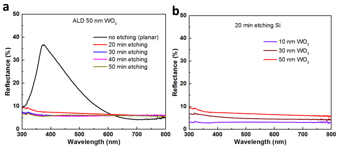
Figure S4: UV-Vis reflectance spectra of (a) WO 3 /Si nanowires with different Si etching time (a) and (b) WO 3 /Si nanowires with different WO 3 film thickness.
