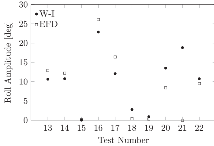
Figure 4.10: Mean roll amplitudes for the cases with \overline{GM} = 1.0 m .
