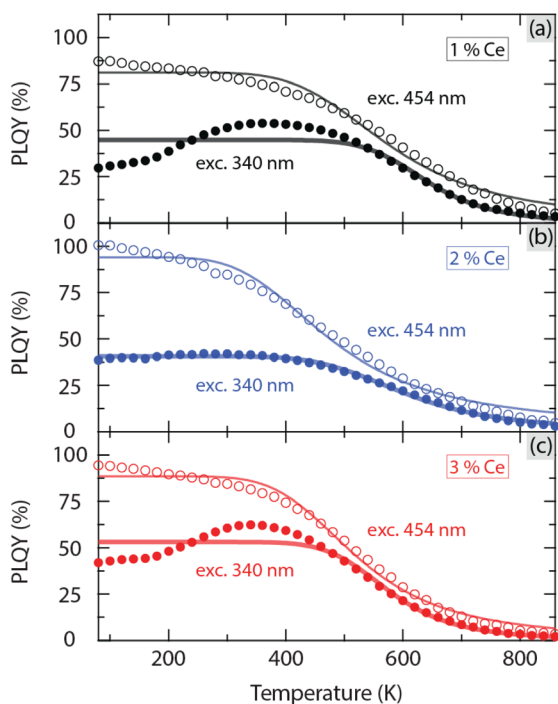
Fig. 3 Variable temperature PLQY of YAG:x%Ce 3+ with x = (a) 1, (b) 2 and (c) 3 for excitation at 454 nm and 340 nm, respectively; see Fig. S2 (ESI†) for luminescence spectra with respect to the one of the excitation source.
