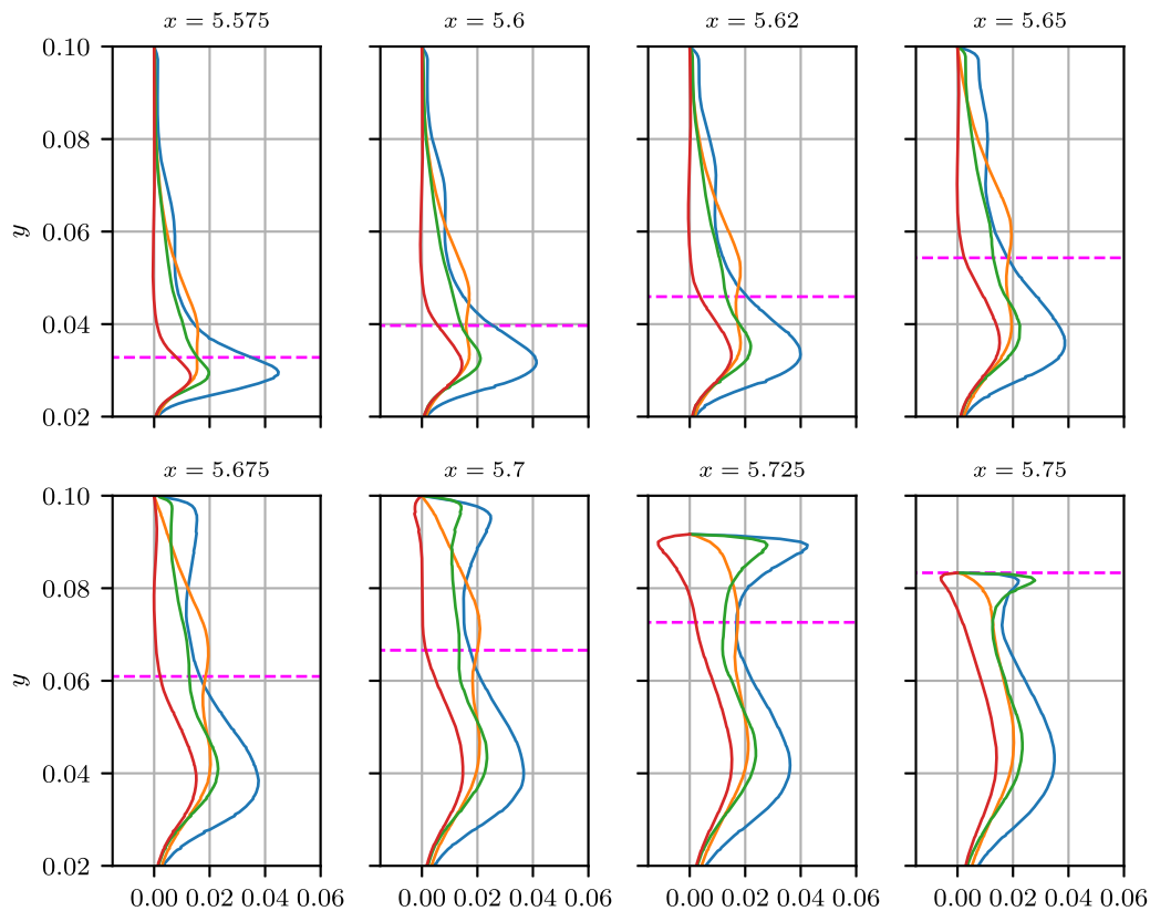
Fig. 11. Profiles of the non-zero components of the \langle u'_i u'_j \rangle tensor at selected values of x close to the beach wall: \langle u'u' \rangle/U_0^2 — blue line, \langle v'v' \rangle/U_0^2 — orange line, \langle w'w' \rangle/U_0^2 — green line, \langle u'v' \rangle/U_0^2 — red line. The magenta dashed line shows the location of the \langle \alpha_{0.5} \rangle isoline. (For interpretation of the references to colour in this figure legend, the reader is referred to the web version of this article.)
