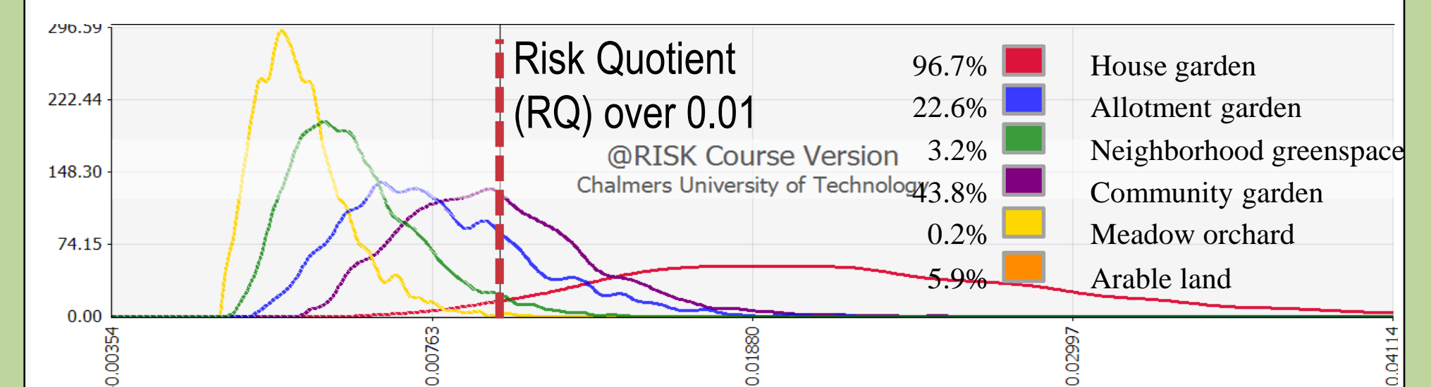
Figure 4: Comparison of acceptable risk for lead (Pb) in UA scenarios for child users (preliminary result with elicited data).
