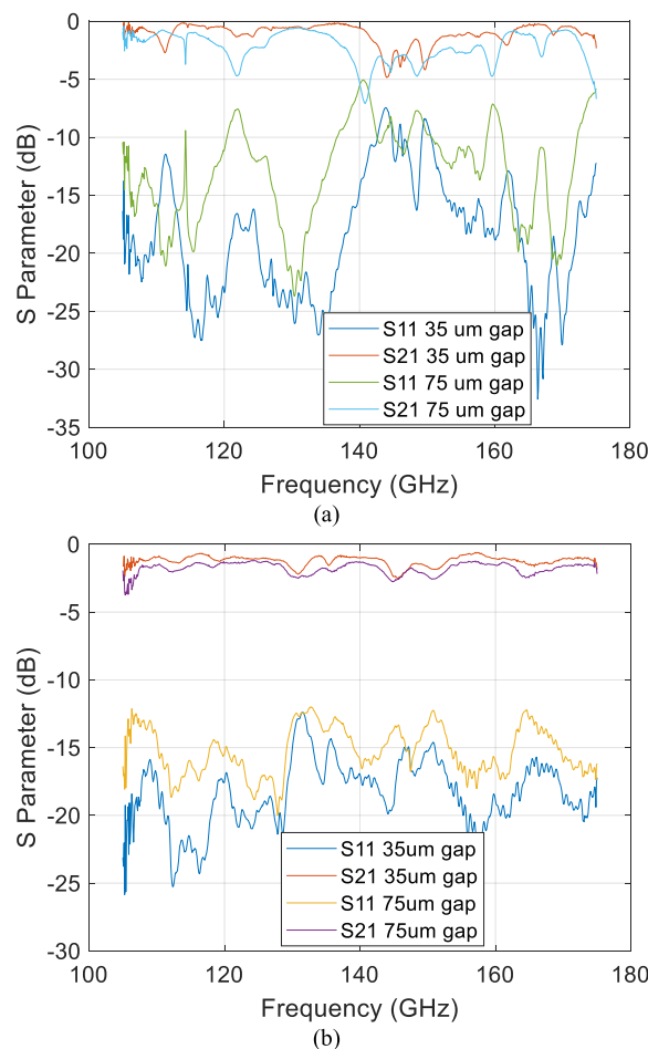
FIGURE 9. Measured S-parameter results: (a) without, and (b) with the proposed EBG structure.
