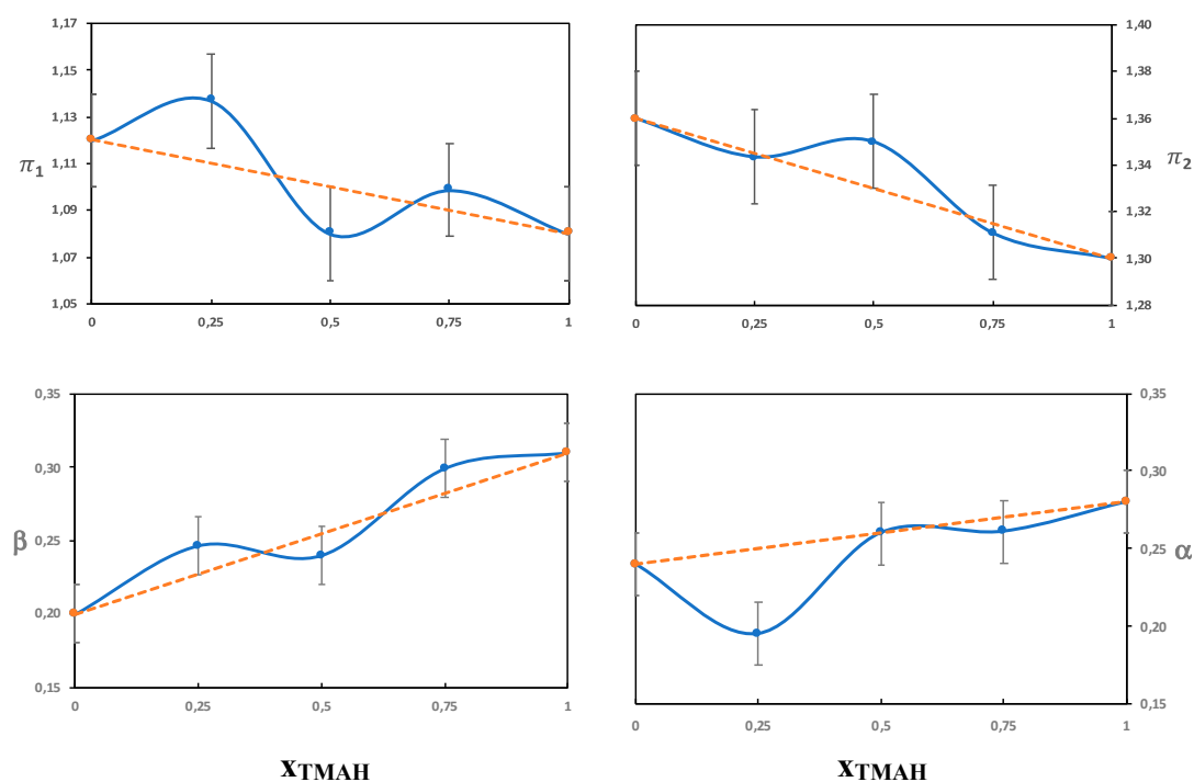
Figure 7. The Kamlet-Taft parameters as a function of the molar fraction of TMAH in solutions of 4 mol% NaOH/TMAH.
