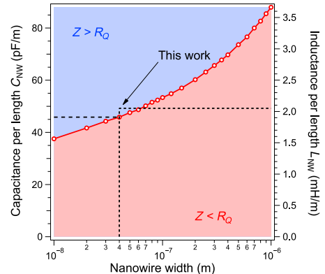
FIG. 8. Simulated capacitance per unit length, C_{NW}(\bar{w}) (red circles), for nanowire widths \bar{w} ranging from 1 \mu\text{m} down to 10 nm. The right axis corresponds to the minimum inductance per unit length, L_{NW}(\bar{w}) , required to obtain a characteristic impedance Z_c = [L_{NW}(\bar{w})/C_{NW}(\bar{w})]^{1/2} > R_Q . The superinductance regime – the area highlighted in blue – should be understood as the range in which L_{NW}(\bar{w}) is sufficiently high, for a fixed \bar{w} , that it will yield Z > R_Q .
