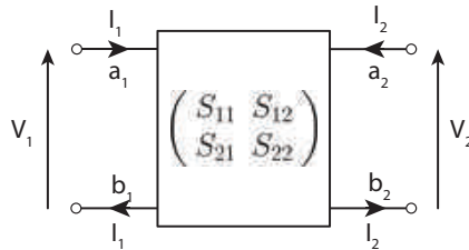
Figure 3.1: Schematic of a two-port network characterised by its scattering matrix. The properties of the two-port network can either be expressed as a function of voltage and current at each port ( V_1 , I_1 , V_2 , I_2 ) or as a function of incident and reflected waves ( a_1 , b_1 , a_2 , b_2 ).
