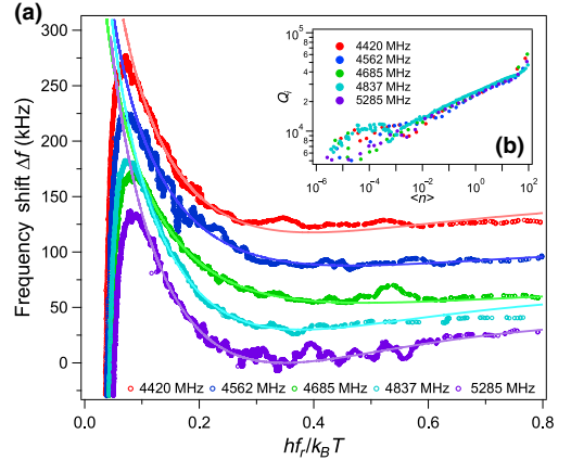
FIG. 4. (a) Frequency shift \Delta f as a function of the normalized frequency f_r of all measured nanowire superinductor resonators. The data is experimentally obtained with the PFLL by tracking the changes in resonant frequency against temperature between 10 mK and 1 K. The solid lines show fits to the theory described by Eq. (2). For clarity, the curves have been offset by 30 kHz. (b) Q_i vs microwave drive power for the same nanowire superinductor resonators (cf. Fig. 3).
