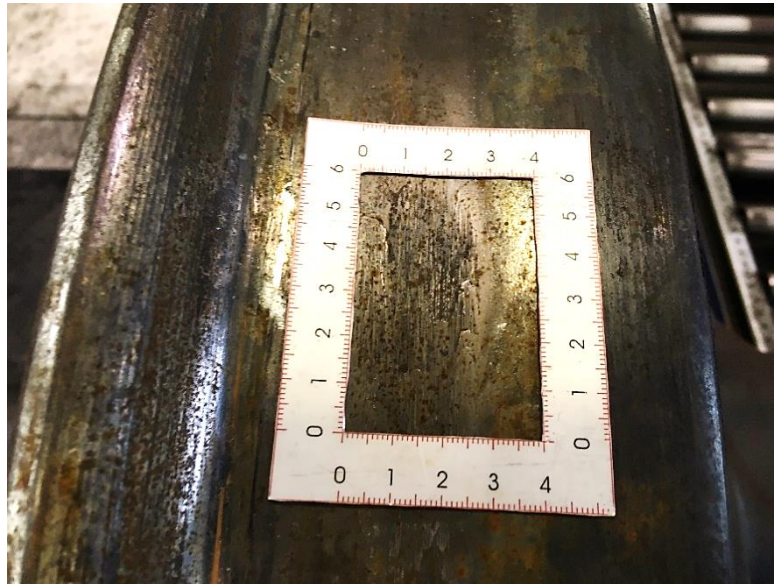
Figure 7: Wheel with a small wheel flat
