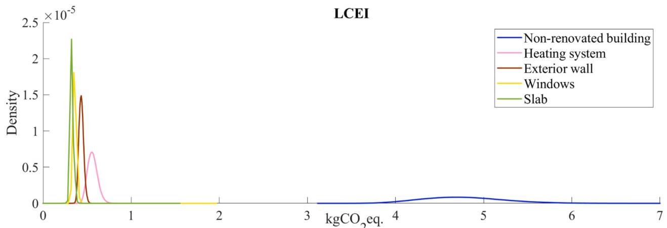
Fig. 4. Results of uncertainty quantification for LCEI in total kg.CO 2 eq.
