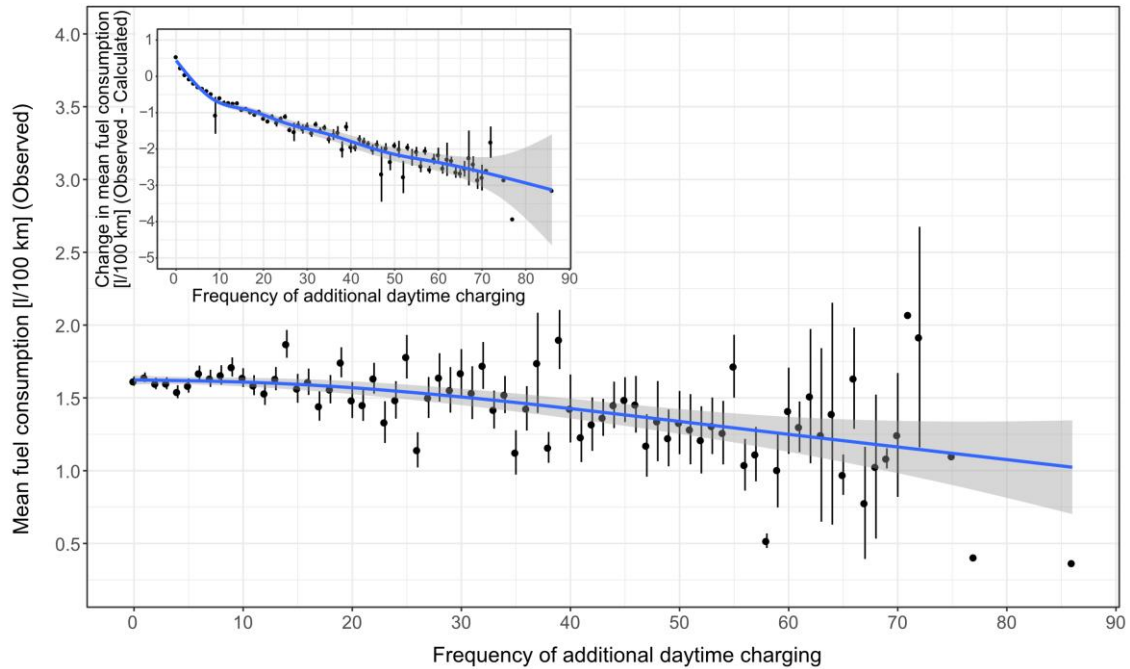
Figure 7: Mean fuel consumption (observed) vs frequency of additional daytime recharging, change in mean fuel consumption (observed-calculated) vs frequency of additional daytime charging given inset. (Paper III)
