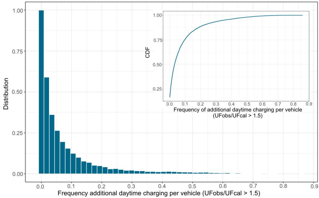
Figure 3: Distribution of additional daytime charging frequency, normalized so maximum is 1. CDF given inset. (Paper II)
