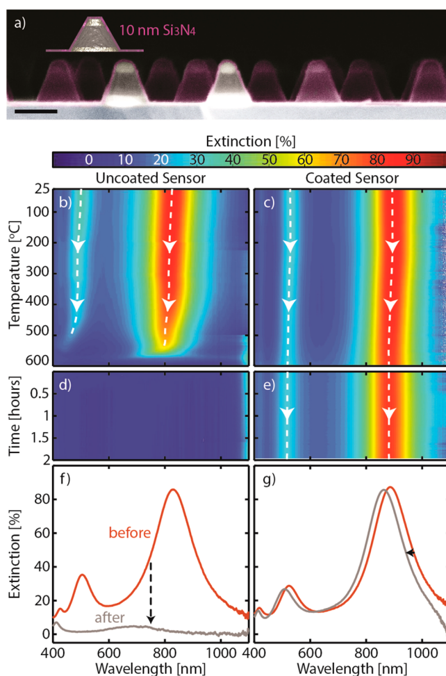
Figure 2. Coating of the 3D metasurface and its stability. (a) False-colored SEM image of a 3D sensor plasmonic metasurface coated with a 10 nm Si 3 N 4 layer (violet). Also shown is the to-scale schematic of the coated sensor. Scale bar is 200 nm. Wavelength-resolved temporal evolution of optical extinction of (b) uncoated and (c) Si 3 N 4 -coated 3D sensors as a function of increasing temperature up to 600 °C under constant flow of 2% O 2 in Ar. The dashed lines denote the spectral peak maximum, \lambda_{\text{peak}} , of the bottom and top disks. For the uncoated sensor, the bottom and top disk LSPR peaks vanish around 500 and 550 °C, respectively, due to complete oxidation. Extended 2 h exposure to 2% O 2 in Ar at 600 °C is also shown for the (d) uncoated and (e) coated sensors. Evidently, the Si 3 N 4 coating excellently protects the Ag nanodisks from oxidation even at very harsh conditions. (f,g) Room temperature extinction spectra of an uncoated and coated metasurface, respectively, before and after the heating/oxidation test.
