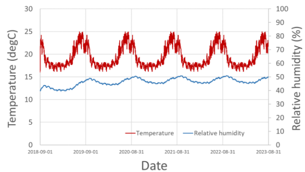
Fig. 18. Calculated temperature and relative humidity inside the wall for 5 years in Lund.
