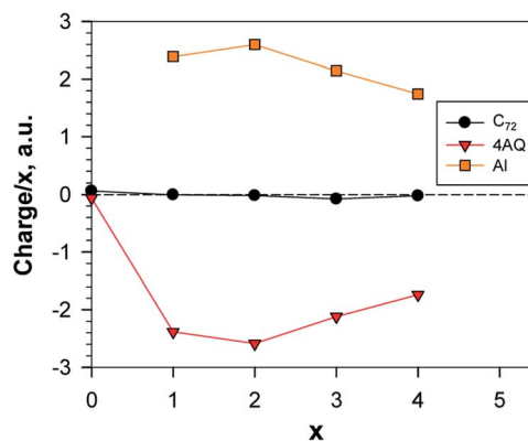
Fig. 16 Normed charges of the Al atoms, the AQs and the graphene; a.u. = 1.6 \times 10^{-19} C; the point x = 0 shows the charge distribution between Gr and \text{AQ}_4 .
