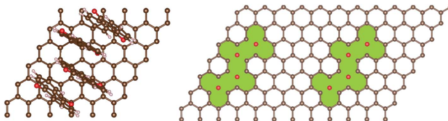
Fig. 4 Top view of the AQ 4 C 72 structure (left) and the π-defect created (right, green).
