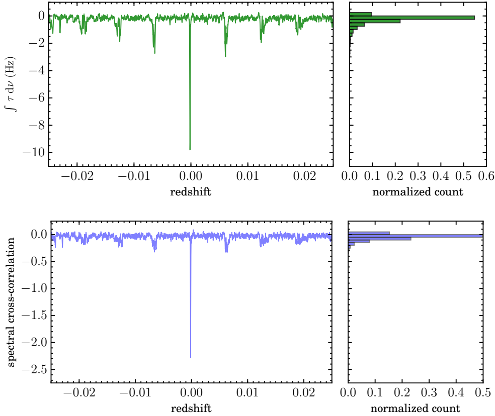
Fig. 4. Cas A spectra cross-correlated for C\alpha RRLs with a template spectrum across a range of redshifts. The plot on the left shows the spectral cross-correlation value at each redshift. The outlying peak at the redshift ( z = -0.000158 ) of the -47 \text{ km s}^{-1} component is again clearly visible. The histogram on the right shows the binned distribution of cross-correlation values. Cas A \alpha -transition stacking demonstrates our method in a regime with a high signal-to-noise ratio.
