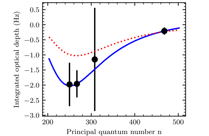
Fig. 12. Integrated optical depth as a function of principal quantum number, n , for the hydrogen RRLs detections associated with the -47\text{ km s}^{-1} velocity component toward Cas A. The figure shows the values from Table 2 using 3\sigma error bars. The blue solid line shows the best-fit model. The red dotted line shows the best-fit model (O17) to carbon RRL detections spanning quantum numbers 225–550 (e.g., see Fig. 10).
