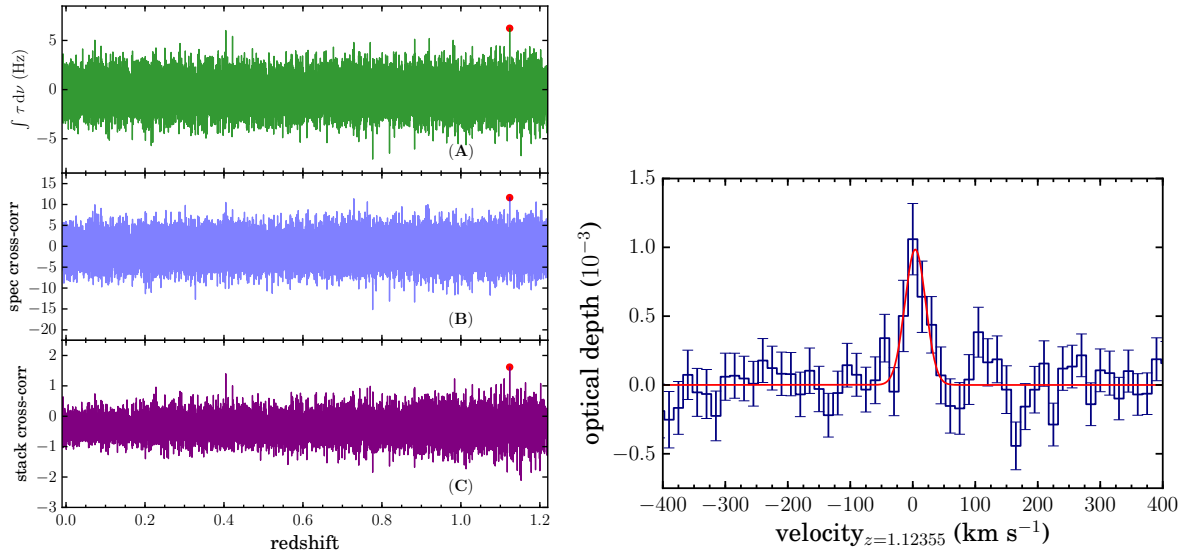
Fig. 15. Our results for 3C 190. Left: same as in Fig. 8, but applied to the \text{Ca}\alpha transitions of 3C 190. The red data point marks the significantly identified redshift of z = 1.12355 . Right: spectrum resulting from stacking \text{Ca}\alpha transitions at z = 1.12355 in 3C 190, using a line-blanking region of \pm 25 \text{ km s}^{-1} .
