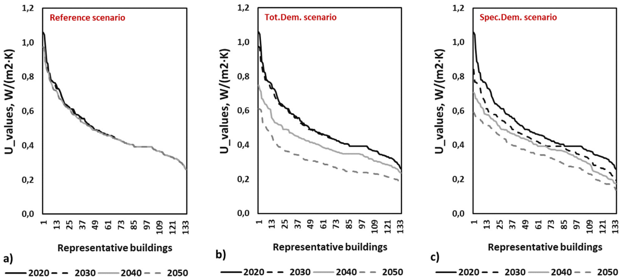
Fig. 4. Overall U-values, sorted in descending order, for the investigated representative buildings of the BS of Gothenburg, as obtained from the modeling of the (a) Reference, (b) Tot.Dem. and (c) Spec.Dem. scenarios. Note that the U-values are sorted in descending order individually for each investment period, which means that the order of the representative buildings in different investment periods is not necessarily the same, and thus, the building numbers cannot be compared between graphs.
