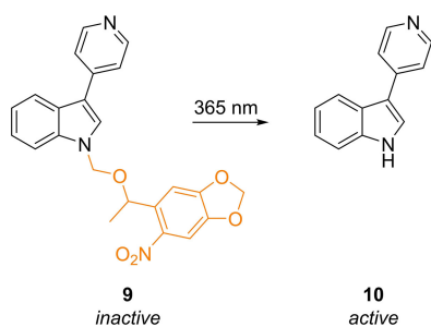
Figure 9. Photoactivation of Rho kinase inhibitor 10 upon irradiation of caged derivative 9 with UV light (365 nm).
