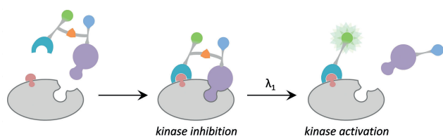
Figure 3. Schematic representation of the active-site directed ‘caging agent’ reported by Lawrence and co-workers. [7]
