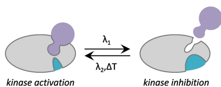
Figure 6. Allosteric control of kinase activity by the inclusion of a LOV2 photosensory domain (blue) into the enzyme. Kinase substrate is depicted in purple.
