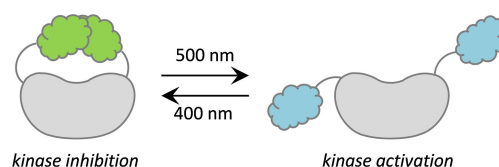
Figure 7. Schematic representation of photoswitchable kinases developed by Lin and co-workers. [16] Figure adapted with permissions from Reference [16], copyright 2017 AAAS.
